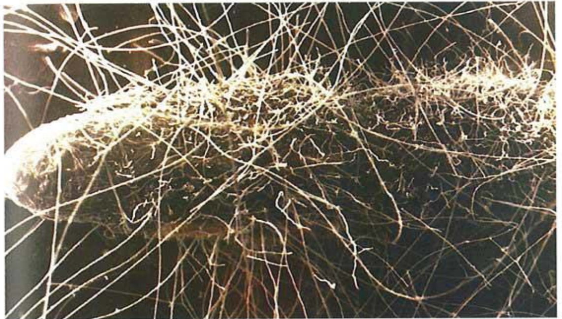
Mycorrhizal fungi, extending from a root—and increasing the plant's ability to obtain nutrients and water. Courtesy Mycorrhizal Applications, www.mycorrhizae.com .
